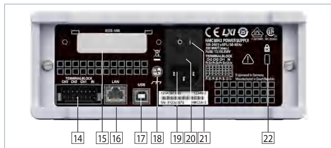
Fig. 2.2: Back panel of R&S®HMC8043
