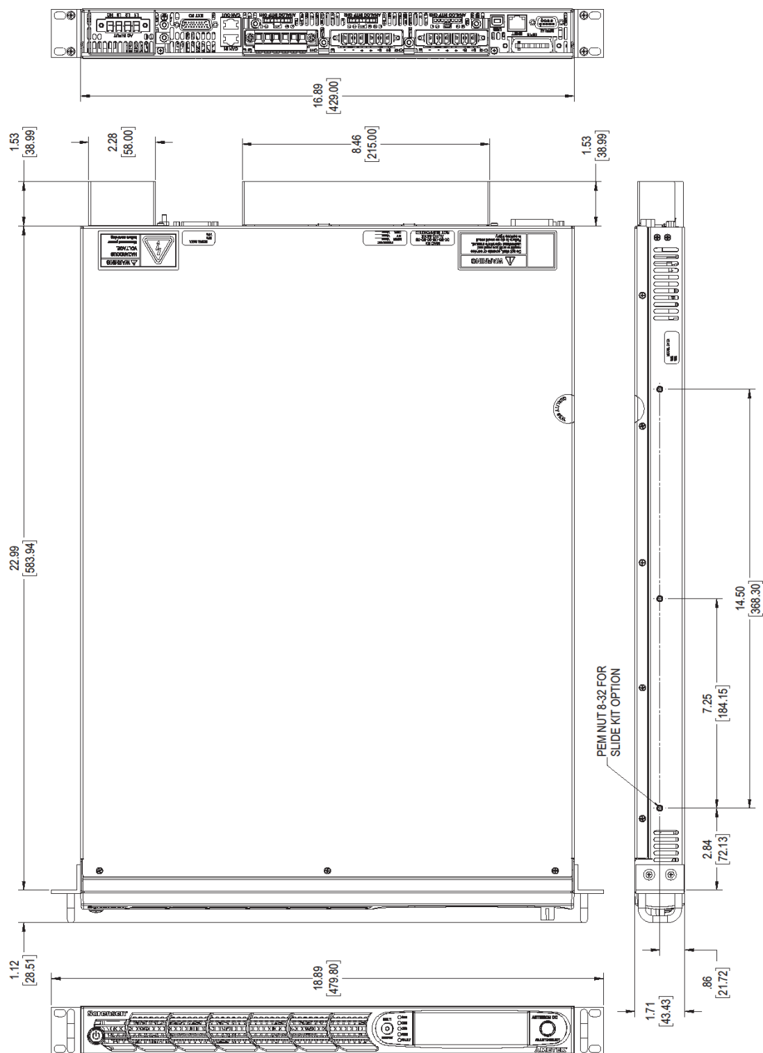
Figure 2-2: Installation Drawing
