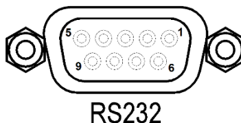
Figure 2-12: RS-232C Interface Connector
