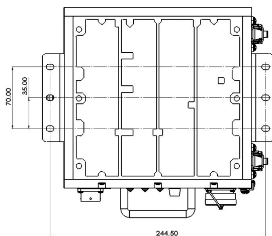
RX-10XX chassis mounting dimensions (in mm)
