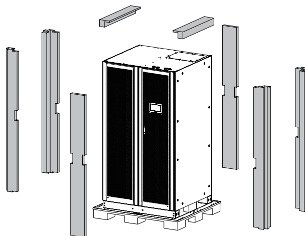
图4-3: 移除缓冲材
