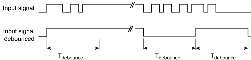
Figure 2-3: Signal curve, debounce input signals
