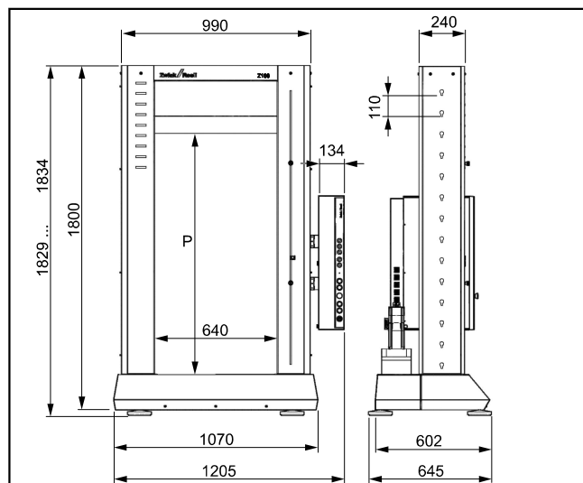
ProLine Z100 TN, Maße
