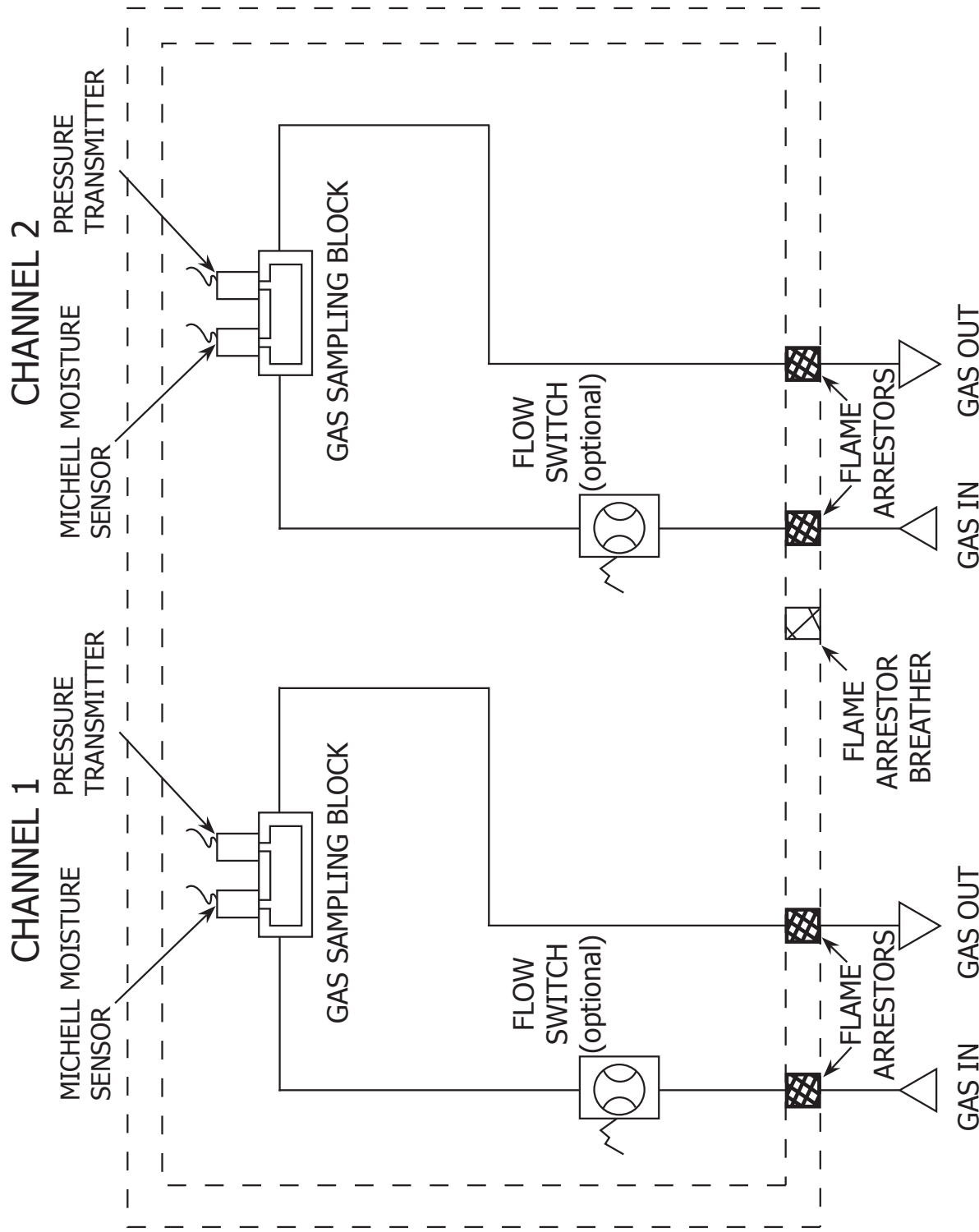
Figure 28 Pipework Connections
