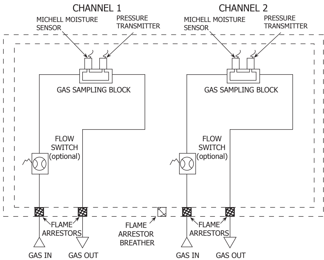
Figure 5 Pipework Connections
