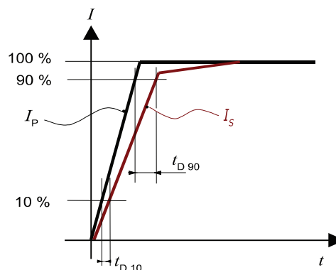
Figure 6: t_{D10} (delay time @ 10 %) and t_{D90} (delay time @ 90 %)
