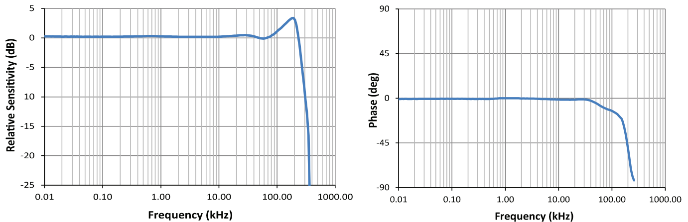
Figures 5 and 6: Typical frequency response, small signal bandwidth
