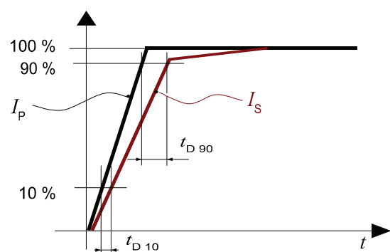
Figure 7: t_{D10} (delay time @ 10 %) and t_{D90} (delay time @ 90 %)
