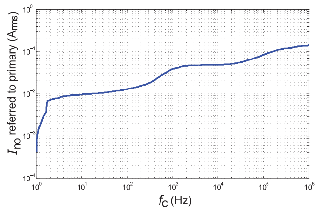
Figure 4: Typical total output current noise with R_M = 100 \text{ } \Omega (primary referred, rms)
