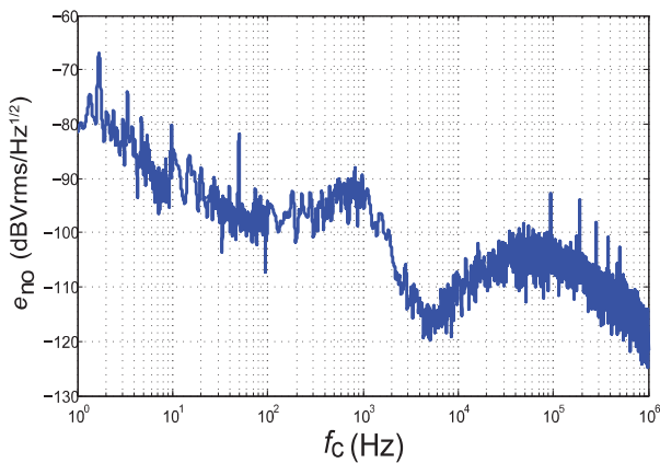
Figure 3: Typical noise voltage density e_{no} with R_M = 100 \text{ } \Omega
