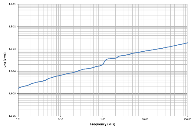
Figure 11: Typical total output RMS noise voltage U_{no} referred to primary
