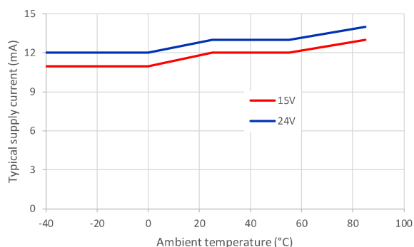
Figure 1: Supply current function of temperature
