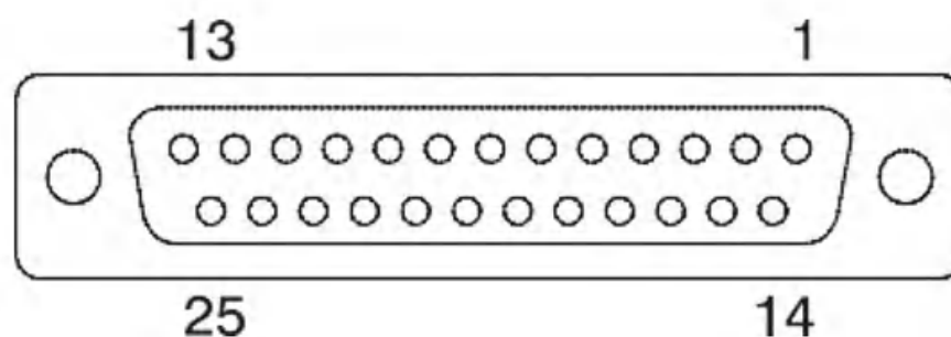
SUB-D 25 female
