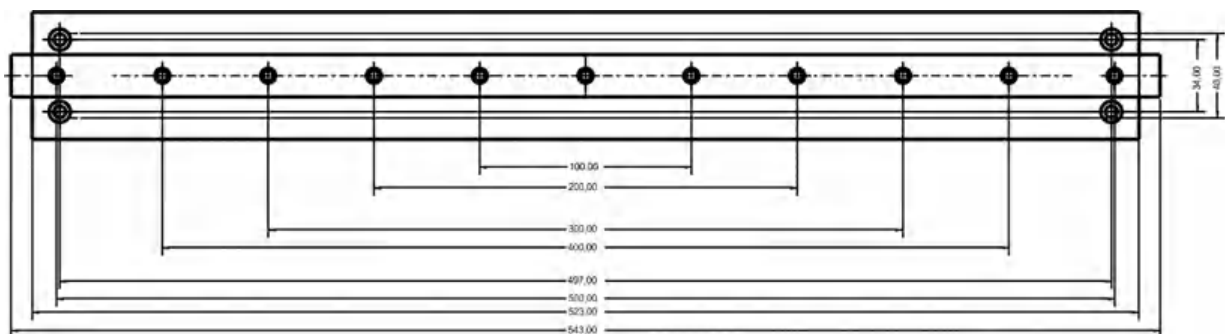
Figure 4-1: Connection to RF reference ground
