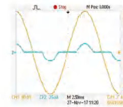
CC mode, CF=2
