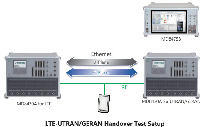
LTE-UTRAN/GERAN Handover Test Setup
