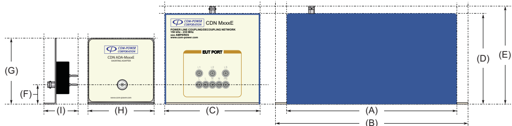
Figure 2 - Product Dimensions
