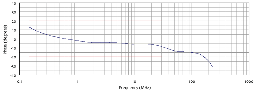
Figure 4 - Typical Phase Data
