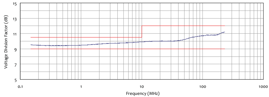
Figure 5 - Typical Voltage Division Factor Data
