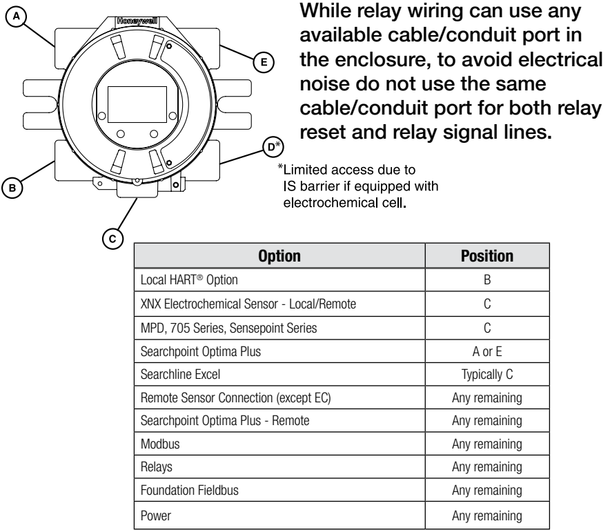
Figure 23. Cable/conduit port assignments
