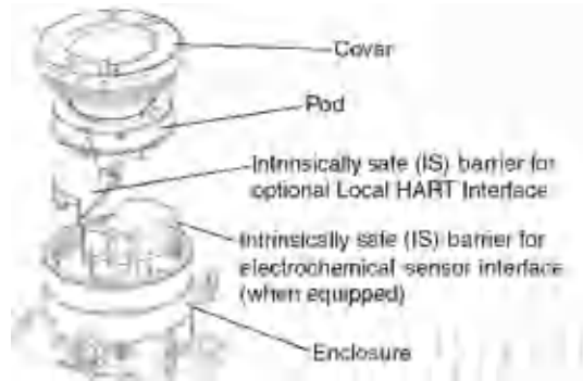
Figure 2. XNX exploded view
