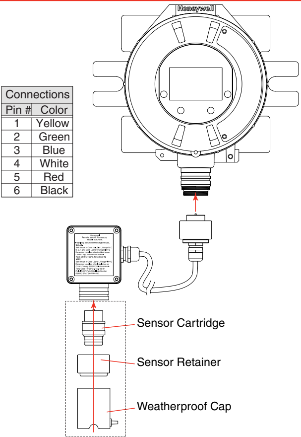
Sensor Mounted to Remote Sensor Kit Figure 42. Installing a remote sensor mounting kit
