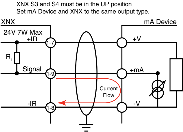
Figure 47. XNX mA input sink configuration
