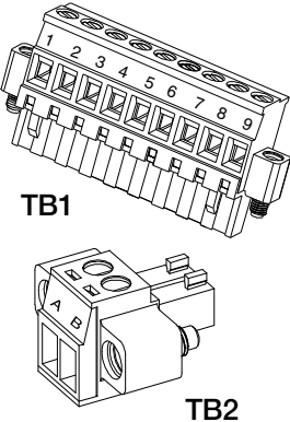
Figure 49. IR personality board terminal blocks, jumper switches and wiring guide
